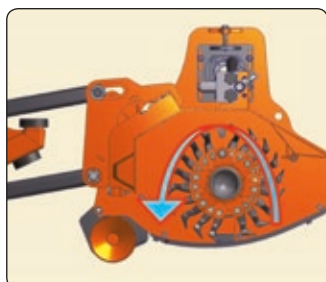
Rotore elicoidale "overlap". "Overlap" rotor.
